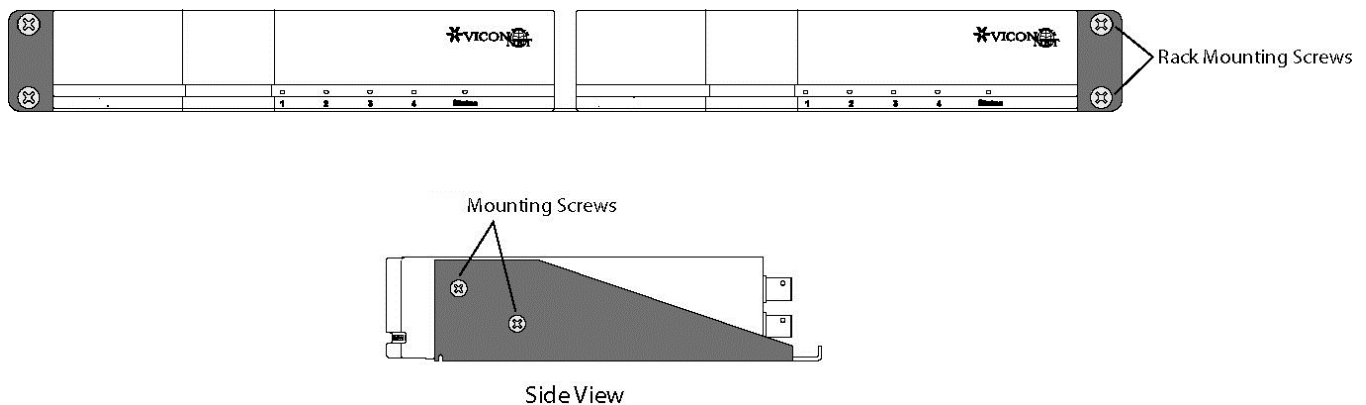
Figure 1 Installing the H264-ENCDCR-RK2
