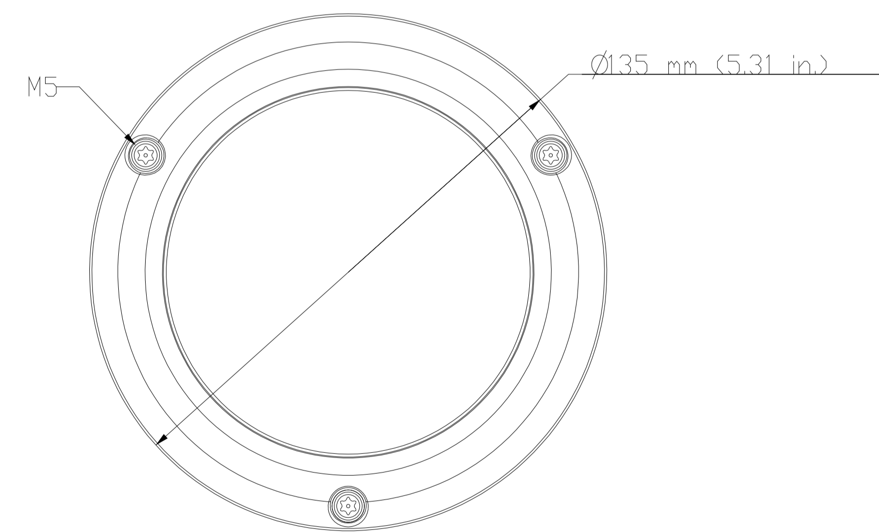
Bottom View
