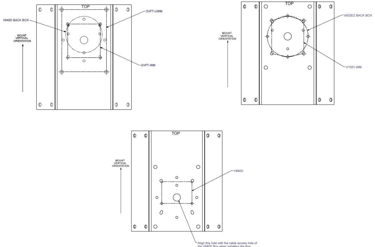
Figure 3 V-24CMB-3 Mounting Holes
