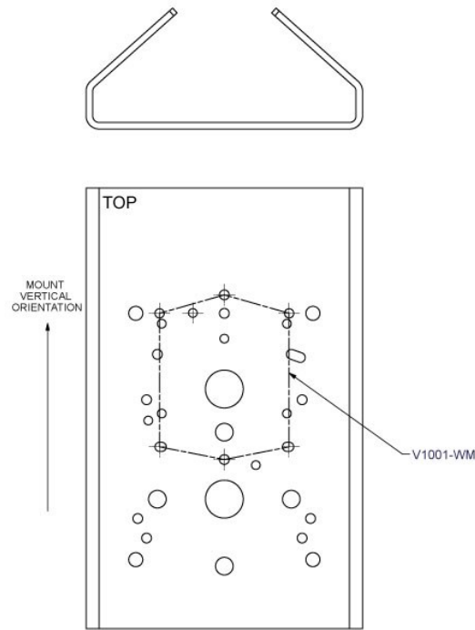
Figure 1 (cont'd) Pole Mounting Adapter Installation
