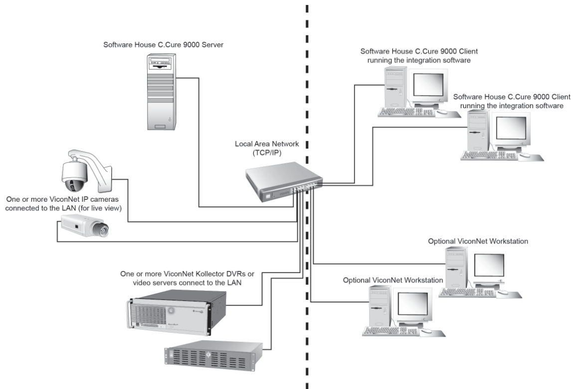
Typical Software House C•Cure 9000/ViconNet Network Setup
